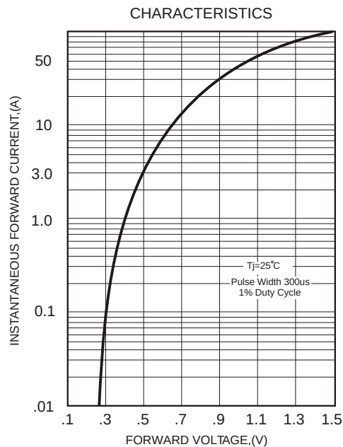
FIG.2-TYPICAL FORWARD
