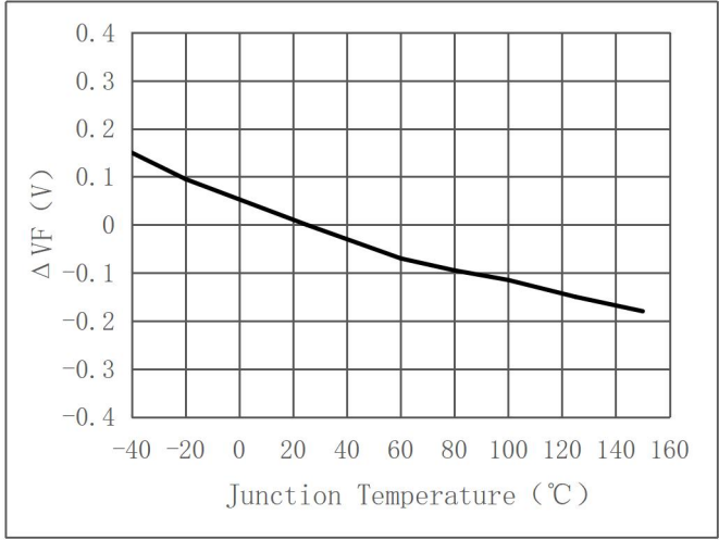
Relative Forward Voltage vs. Junction Temperature ( \Delta VF = VF - VF(25^\circ C) = f(T_j) @ I_F = 200mA )
