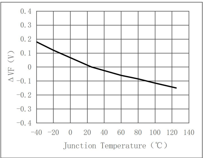
Relative Forward Voltage vs. Junction Temperature ( \Delta VF=VF-VF(25℃)=f(Tj) @IF=50mA)
