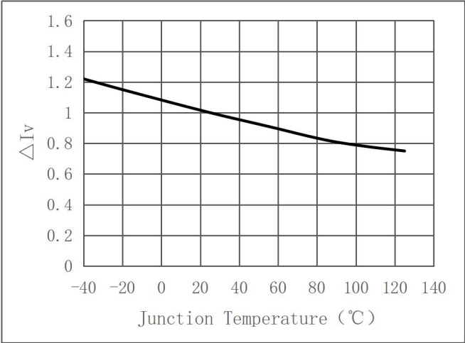
Relative Luminous Intensity vs. Junction Temperature ( \Delta I_v = I_v / I_v(25^\circ\text{C}) = f(T_j) IF=50mA)
