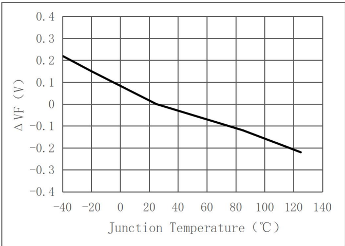
Relative Forward Voltage vs. Junction Temperature ( Δ VF=VF-VF(25℃)=f(Tj) @IF=50mA )
