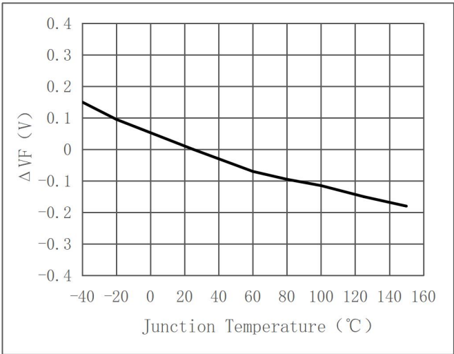
Relative Forward Voltage vs. Junction Temperature ( Δ VF=VF-VF(25℃)=f(Tj) @IF=200mA )
