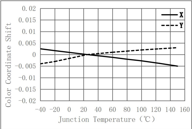
Junction Temperature vs. Color Coordinate Shift ( \Delta C_x, \Delta C_y = f(T_j) ; IF = 200 mA) (Amber)
