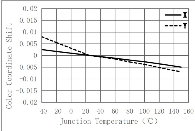
Junction Temperature vs. Color Coordinate Shift ( \Delta C_x, \Delta C_y = f(T_j) ; IF = 200 mA) (White)
