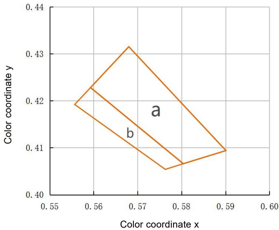
Bin Range of Chromaticity Coordinates Specifications
