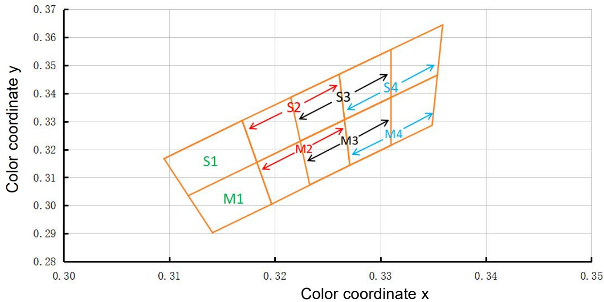
Bin Range of Chromaticity Coordinates Specifications
