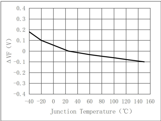
Relative Forward Voltage vs. Junction Temperature ( \Delta VF=VF-VF(25^\circ C)=f(T_j) @IF=350mA )
