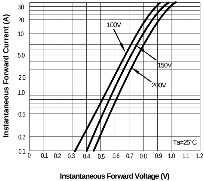
FIG3: Forward Voltage
