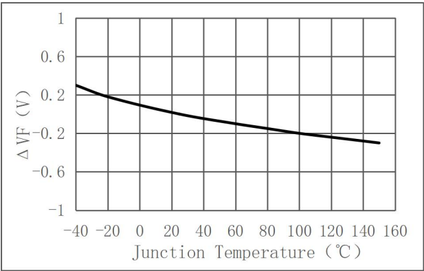
Relative Forward Voltage (Red \Delta VF )
