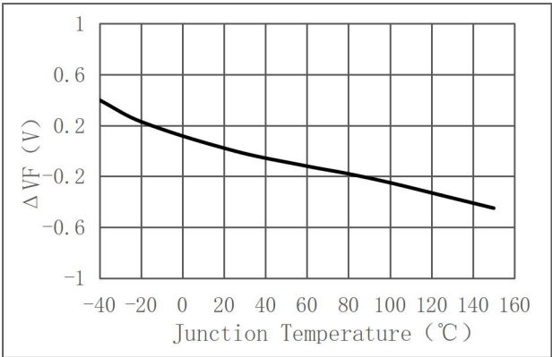
Relative Forward Voltage (Green \Delta VF )
