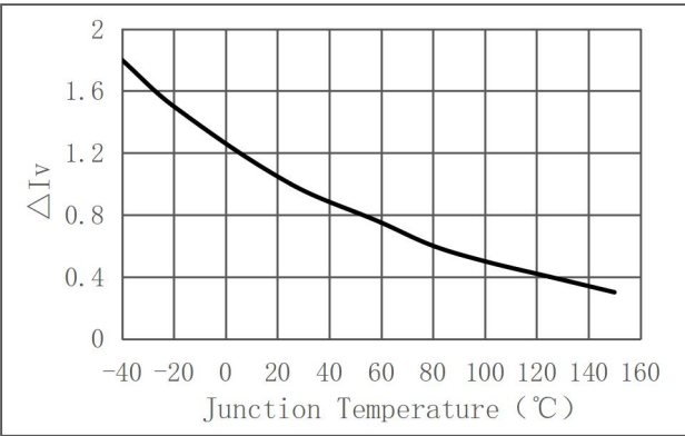
Fluctuations in relative luminous intensity (Blue \Delta IV=IV/IV )
