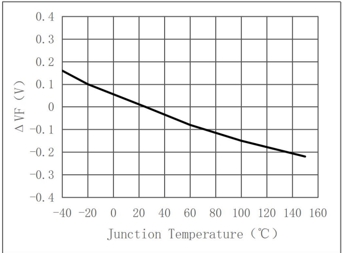
Relative Forward Voltage vs. Junction Temperature ( \Delta V_F = V_F - V_F(25^\circ \text{C}) = f(T_j) @IF=200mA)
