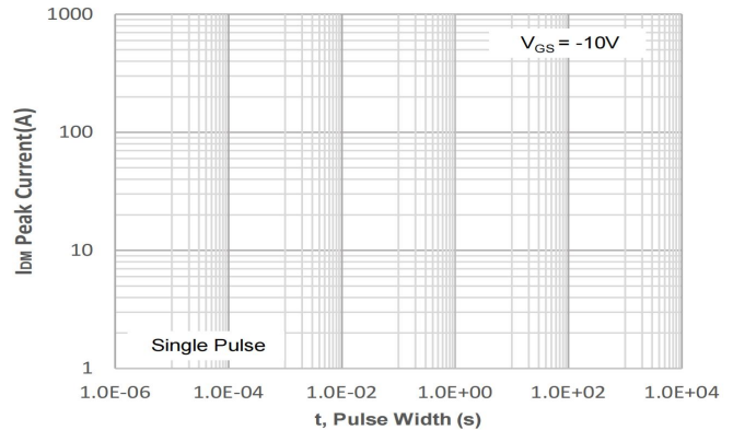
Figure 12: Peak Current Capacity
