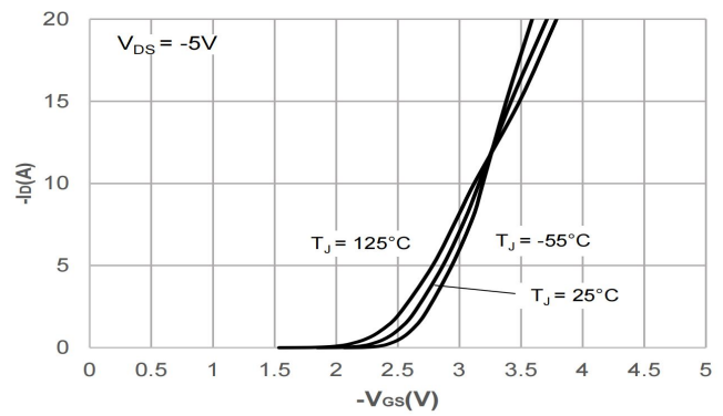
Figure 2: Typical Transfer Characteristics
