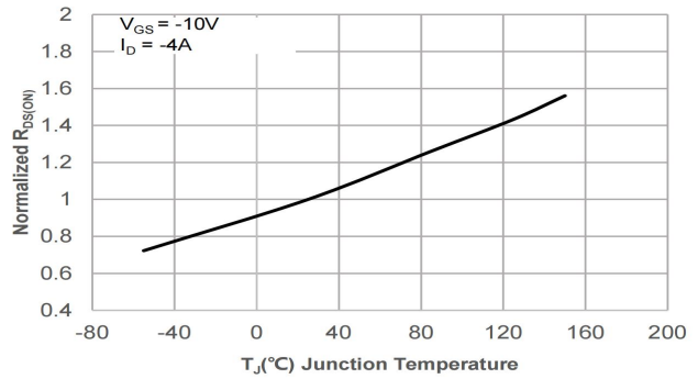
Figure 8: Normalized on Resistance vs. Junction Temperature
