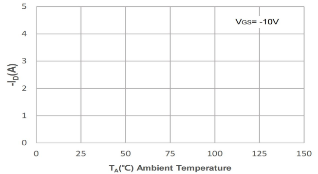
Figure 10: Maximum Continuous Driain Current vs. Ambient Temperature
