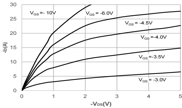
Figure 1: Output Characteristics
