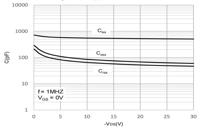
Figure 6: Capacitance Characteristics
