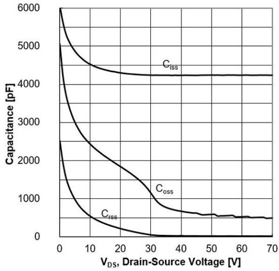
Figure 12. Capacitance Characteristics
