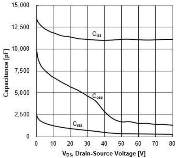
Figure 12. Capacitance Characteristics
