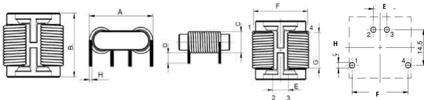
Inductor Dimensions (mm)
