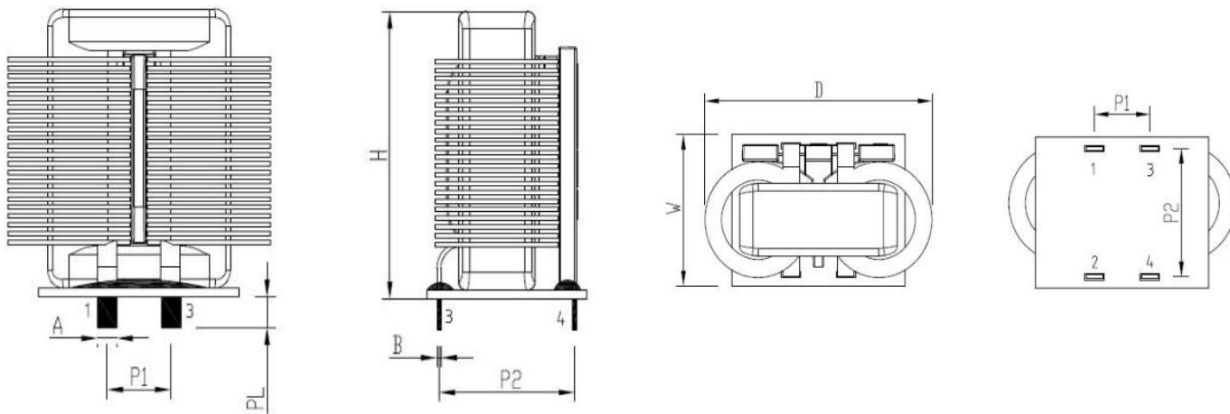
Inductor Dimensions (mm)
