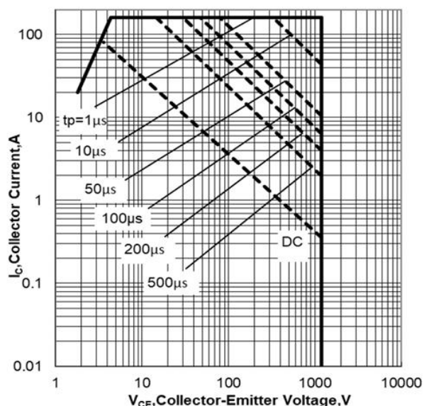
Figure 1. Forward Bias Safe Operating Area
