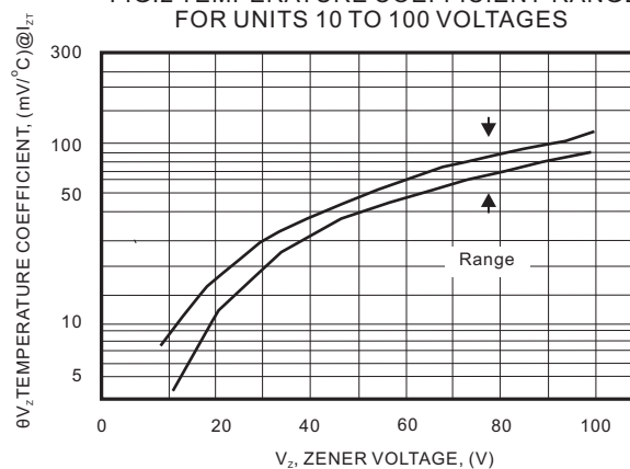
FIG.2 TEMPERATURE COEFFICIENT-RANGE FOR UNITS 10 TO 100 VOLTAGES
