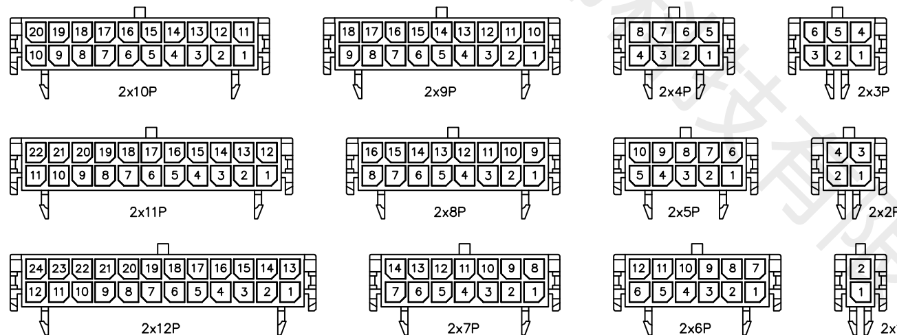
CIRCUIT SIZE LAYOUT
