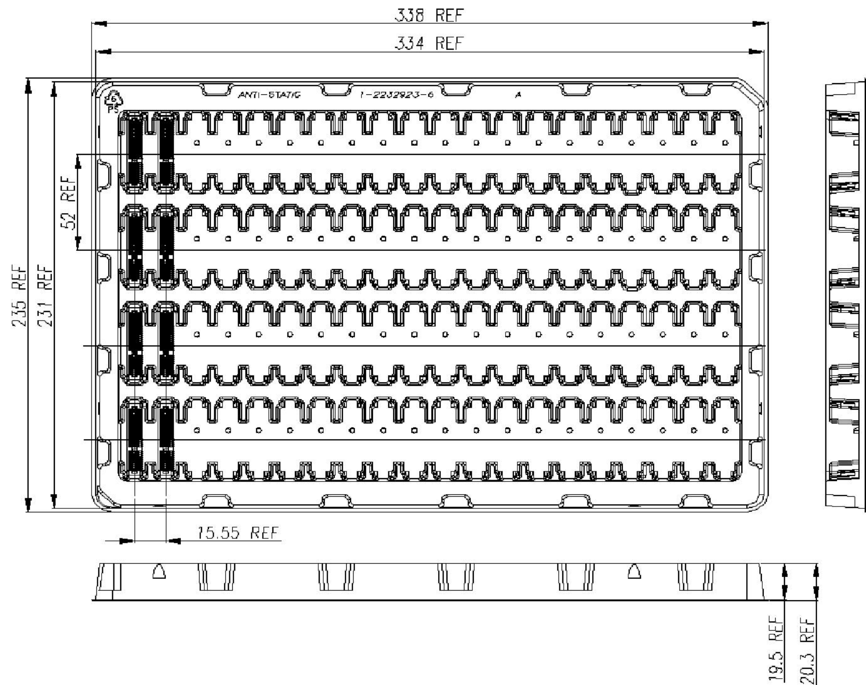
SOFT TRAY: FOR 64POS SCALE: 1:2
