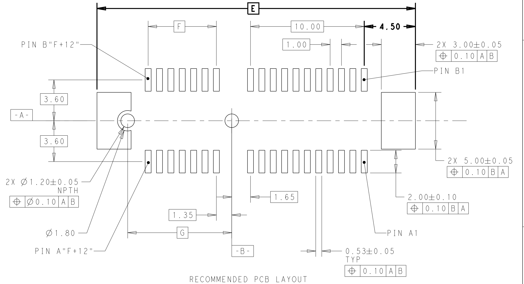
RECOMMENDED PCB LAYOUT
