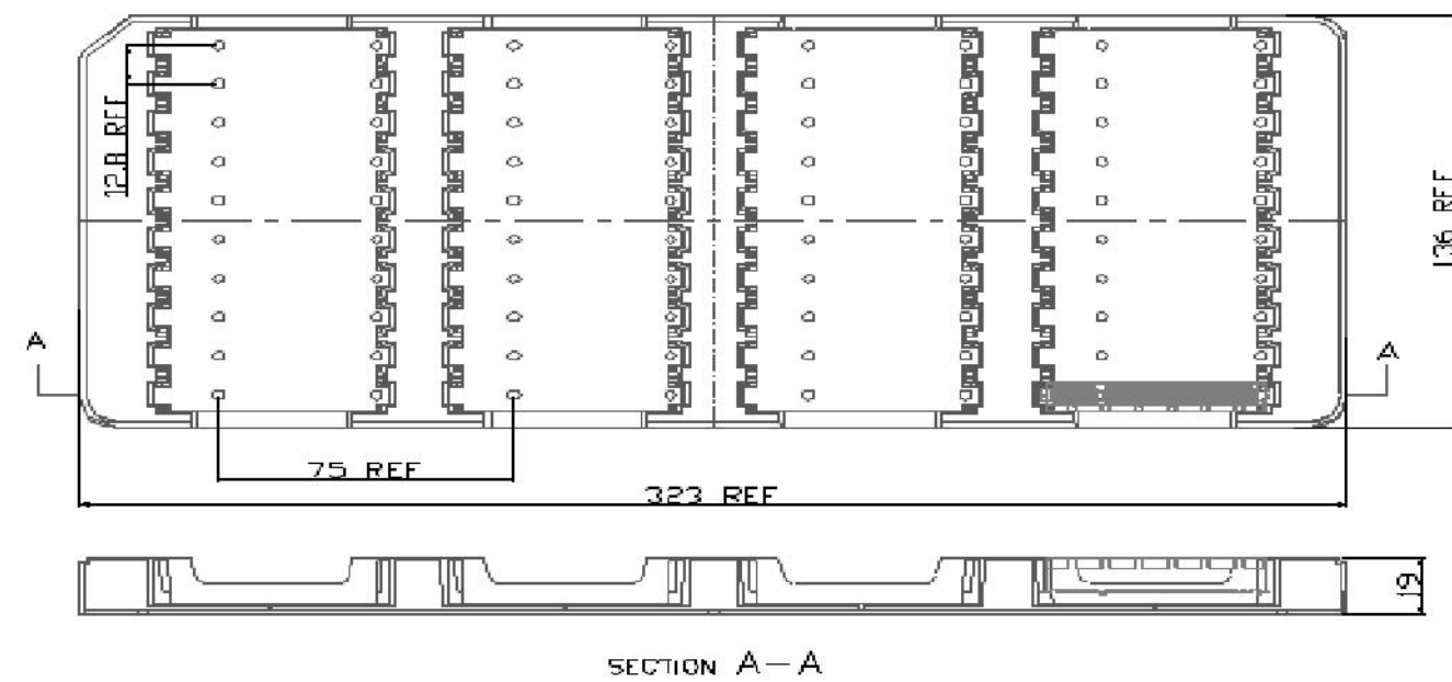
HARD TRAY: FOR 6-2364427-7 (98POS) SCALE: 1:2
