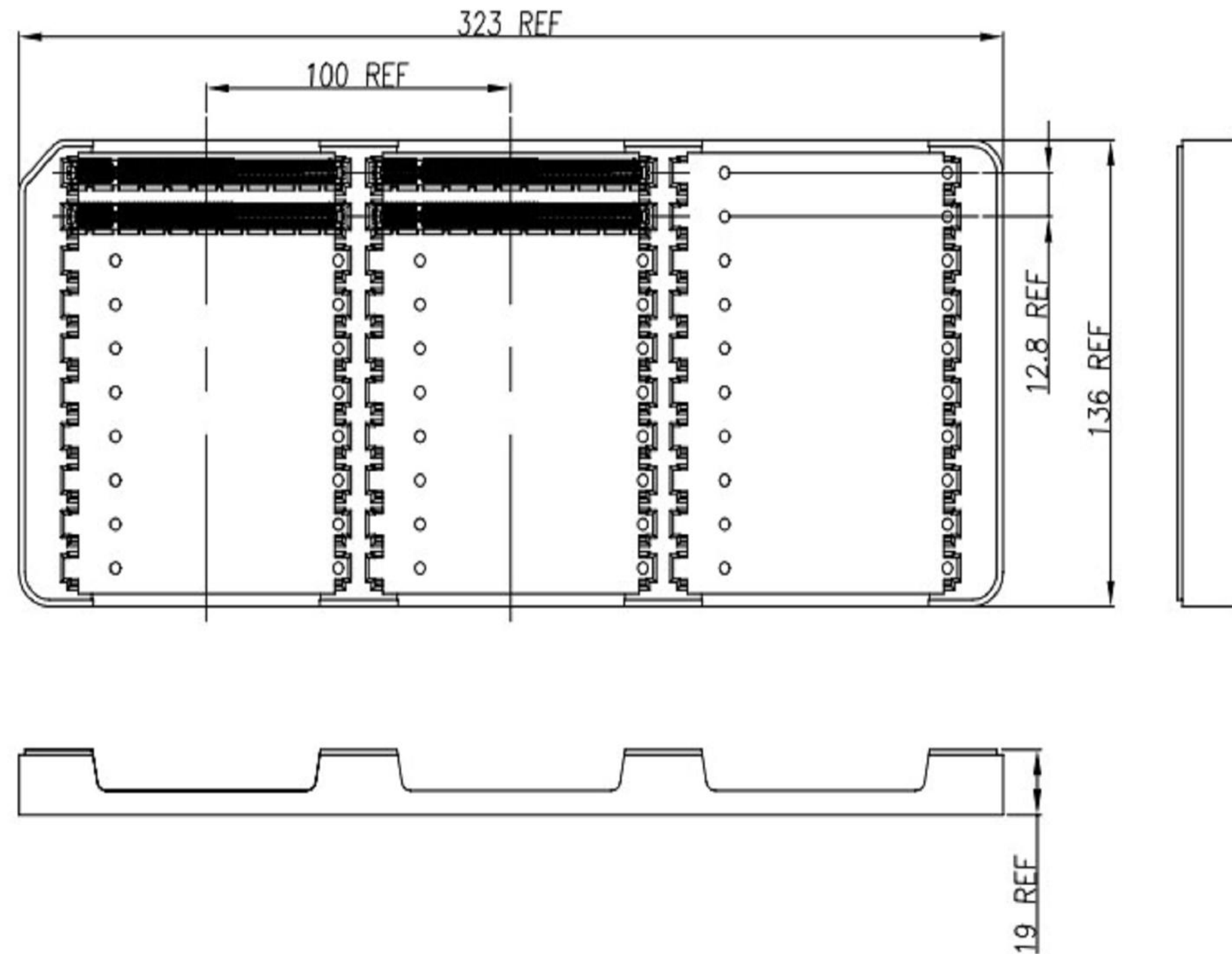
HARD TRAY: FOR 6-2364427-8/9 AND 4-2364427-9 (164POS) SCALE: 1:2
