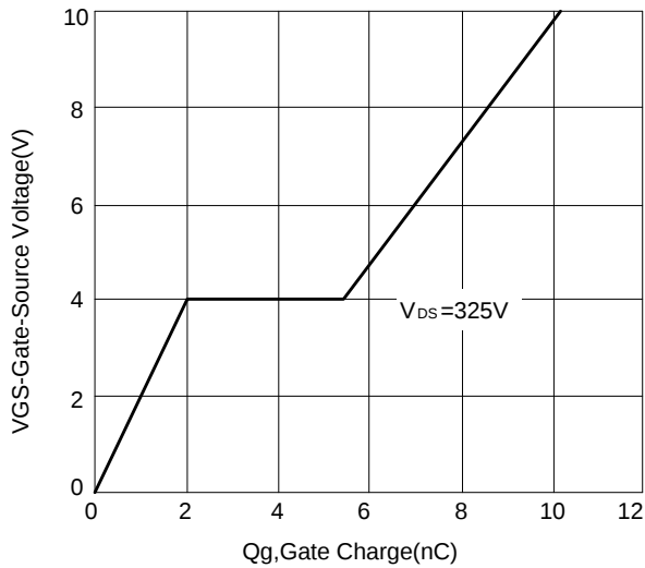
Figure 9: Gate Charge vs Gate to Source Voltage
