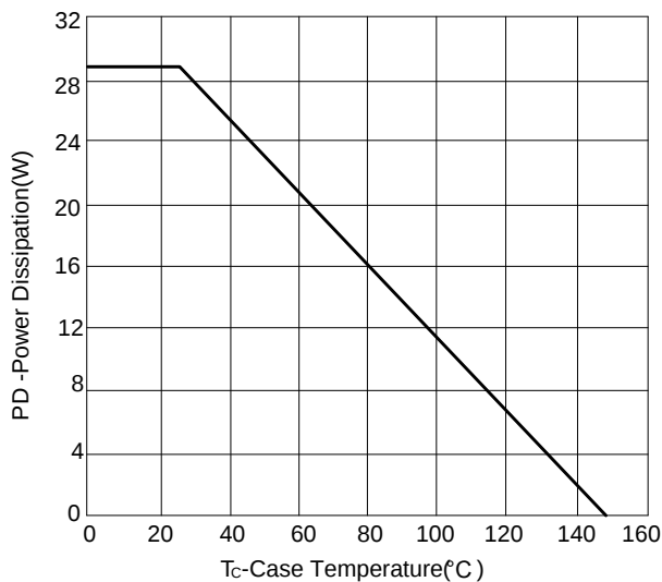
Figure 11: Power Dissipation vs Case Temperature
