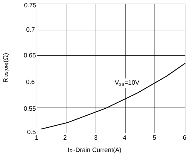
Figure 3: Drain to Source On-Resistance vs Drain Current
