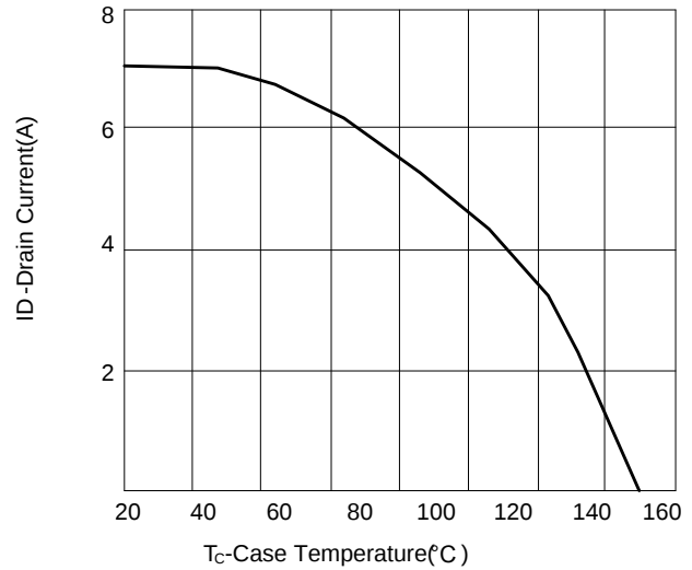
Figure 10: Continuous Drain vs Case Temperature
