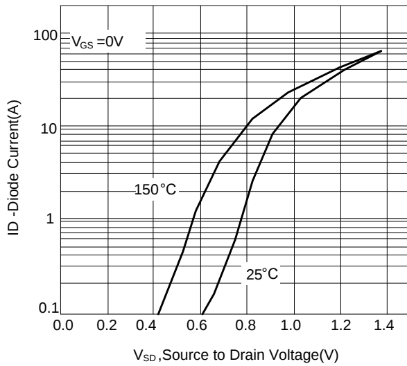
Figure 7: Body Diode Characteristics
