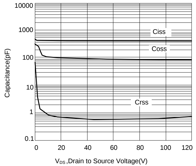
Figure 8: Capacitance vs Drain to Source Voltage
