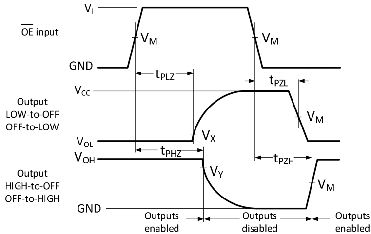
Fig. 6. 3-state enable and disable times
