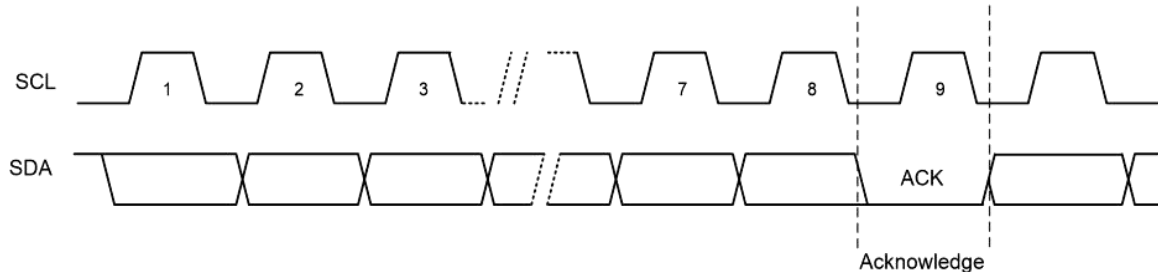
Figure 4-3 Output Acknowledge
