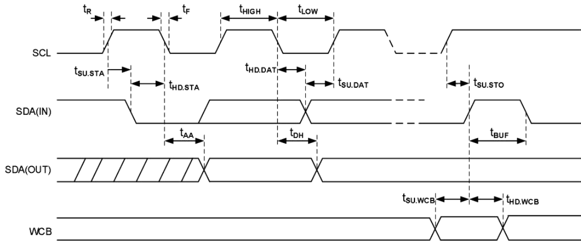
Figure 3-1 Bus Timing
