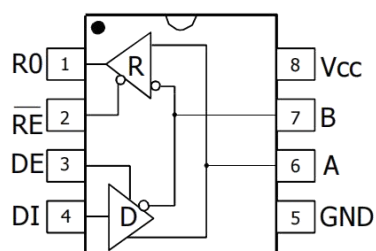
DIP-8/SOP-8/MSOP-8
