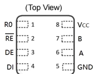
DFN-8 3*3
