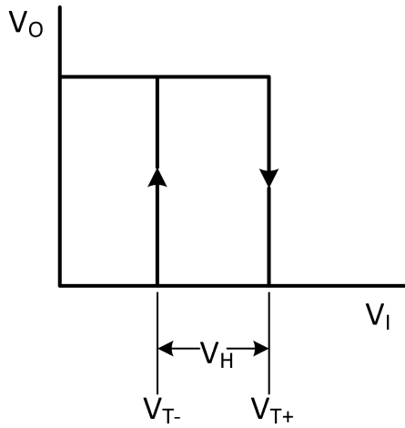
Fig. 12. Transfer characteristic
