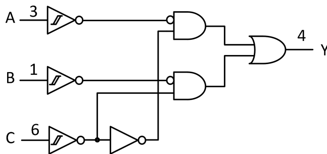
Fig. 1. Logic symbol
