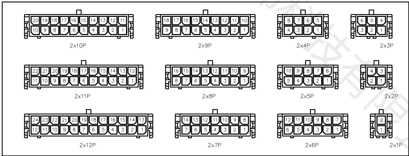
CIRCUIT SIZE LAYOUT
