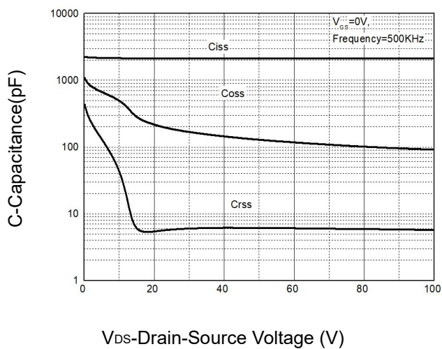
Figure 9: Capacitance Characteristics
