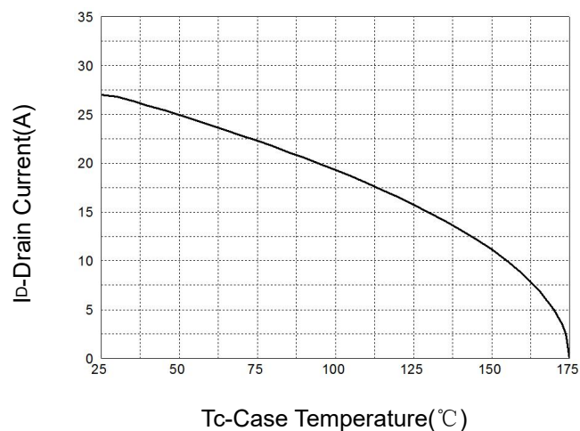
Figure 2: Drain Current
