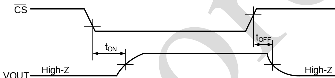
开启/关断时序 (AiP8623)
