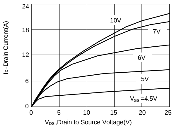
Figure 10: Output Characteristics
