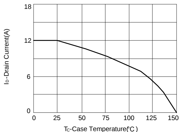
Figure 9: Continuous Drain vs Case Temperature
