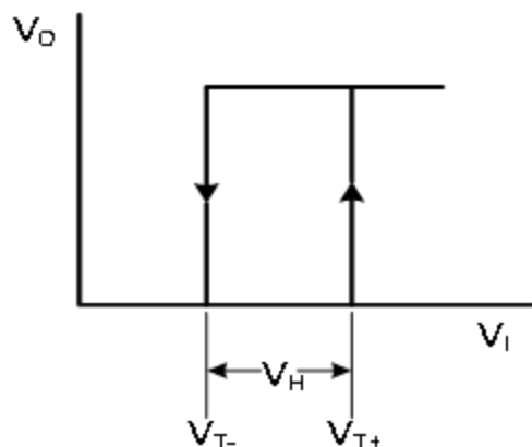
Fig 8. Transfer characteristic
