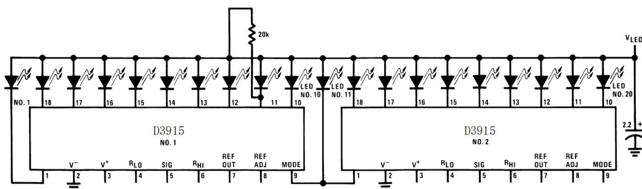
Cascading D3915s in Dot Mode
