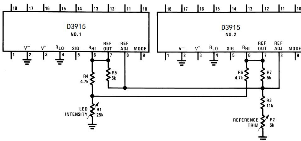
FIGURE 9. Independent Adjustment of Reference Voltage and LED Intensity for Multiple D3915s
