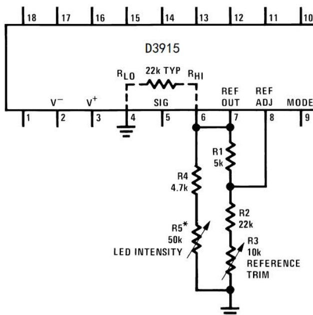
FIGURE 8. Varying LED Intensity
