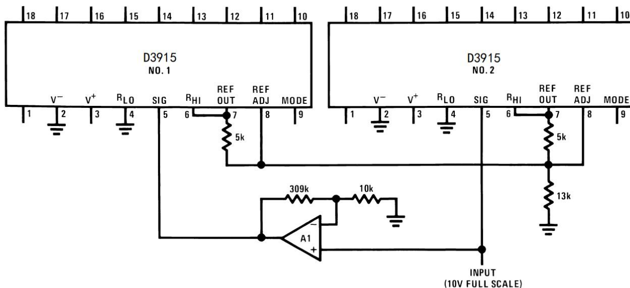
FIGURE 6. Improved Circuit for 60 dB Display
