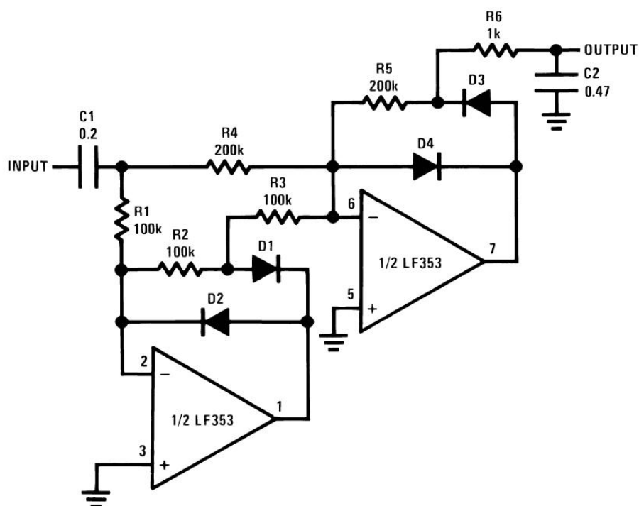
FIGURE 3. Precision Full-Wave Average Detector
