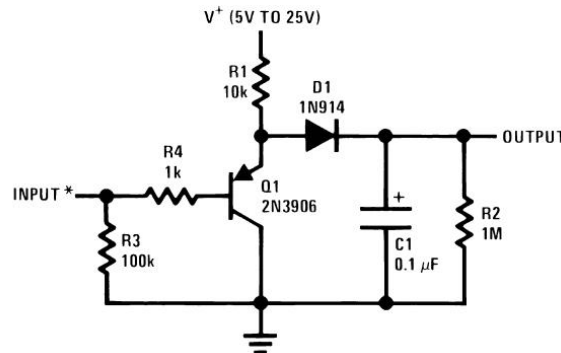
FIGURE 1. Half-Wave Peak Detector
