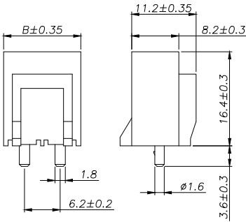
2 Pin
