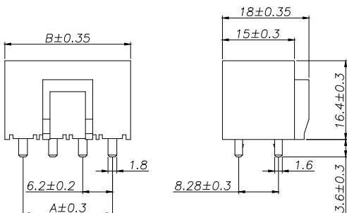
2x4 Pin
