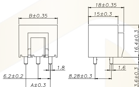
2x3 Pin
