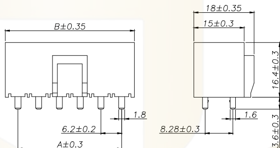
2x6 Pin
