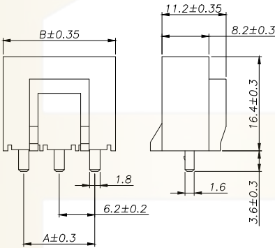
3 Pin
