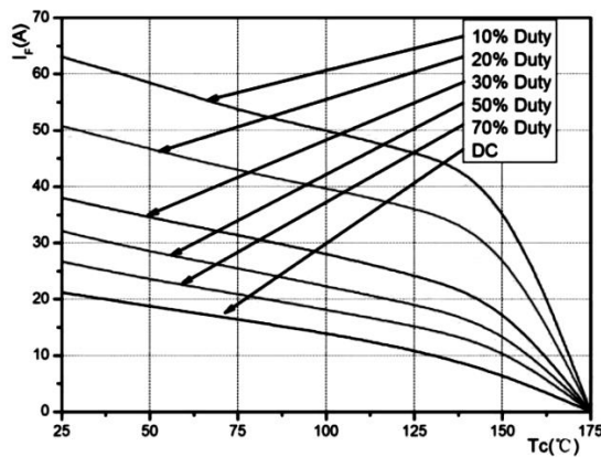
Figure 3. Load current
