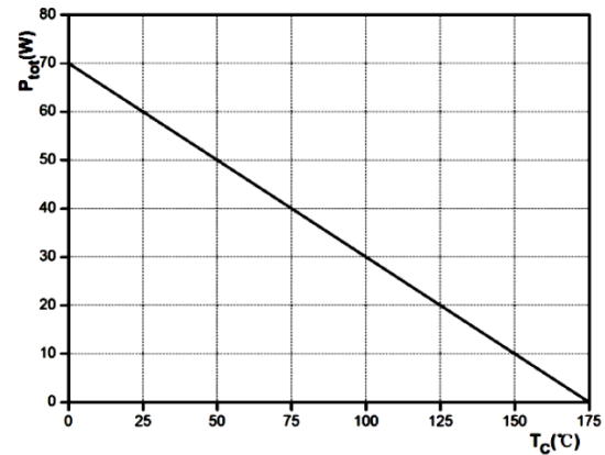
Figure 4. Dissipated power curve
