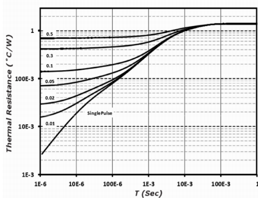
Figure 6. Thermal Impedance Junction-to-Case
