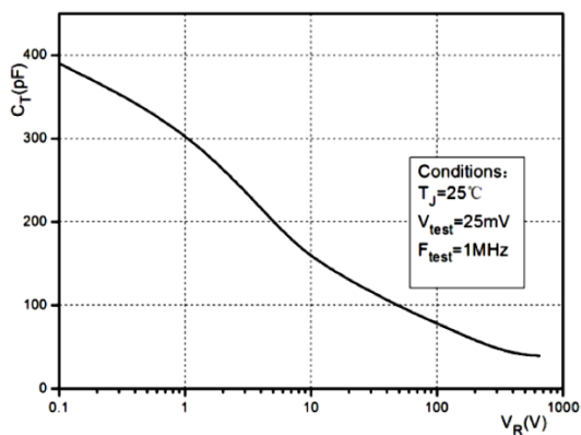
Figure 5. Capacitance vs reverse voltage
