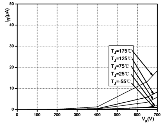
Figure 2. Reverse Characteristics
