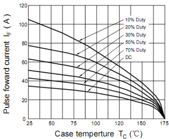
Figure 3. Current Derating
