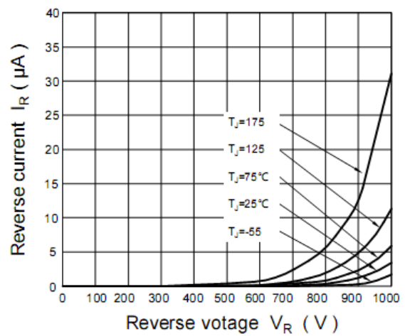
Figure 2. Reverse Characteristics
