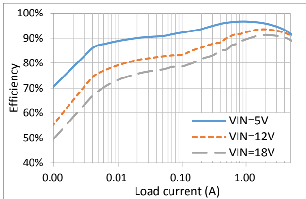
Figure 1. Efficiency vs Iout (V OUT = 3.3V, L = 2.2uH)
