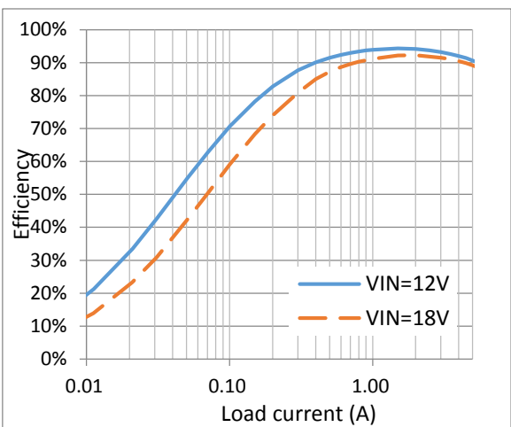
Figure 8. Efficiency vs Load Current (V OUT =5V, L=3.3uH)
