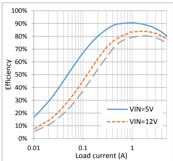
Figure 9. Efficiency vs Load Current (V OUT =1V, L=1uH)
