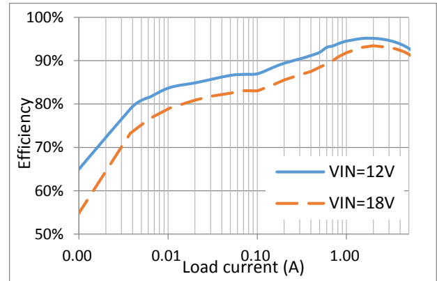
Figure 2. Efficiency vs Iout (V OUT = 5V, L = 3.3uH)
