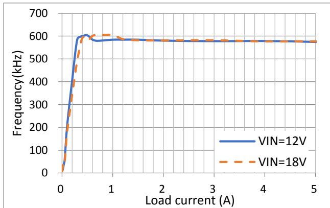
Figure 3. Frequency vs Iout (V OUT = 3.3V, L = 2.2uH)
