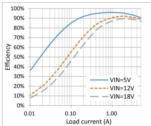
Figure 7. Efficiency vs Load Current (V OUT =3.3V, L=2.2uH)
