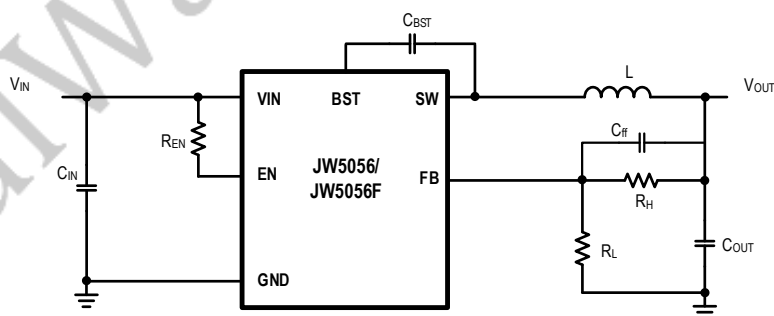
18V/5A Step Down Regulator
