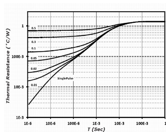
Figure 6. Thermal Impedance Junction-to-Case
