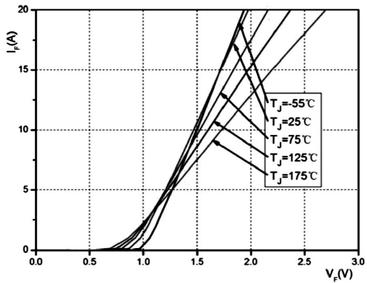
Figure 1. Forward Characteristics
