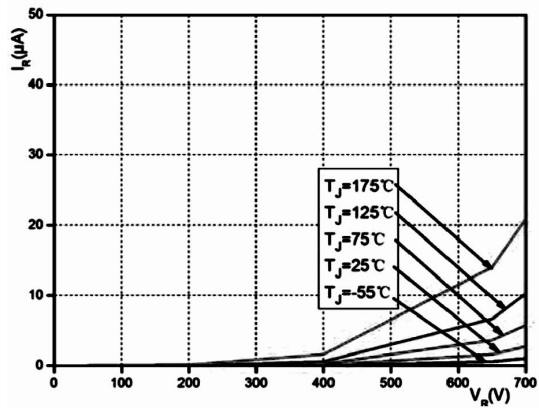
Figure 2. Reverse Characteristics
