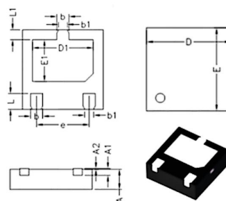
DFN2020-3L
