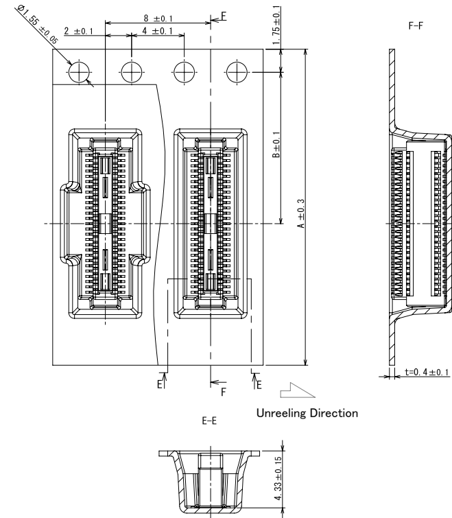
Embossed Tape Dimensions
