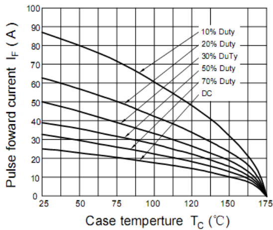
Figure 3. Current Derating
