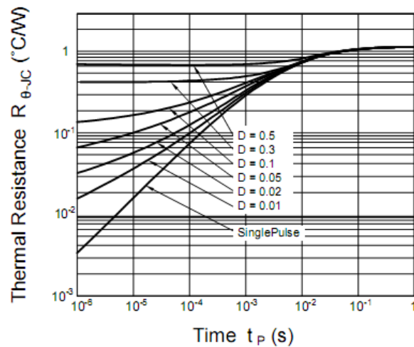
Figure 6. Thermal Impedance Junction to Case
