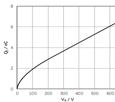
Figure 6. Total Capacitance charge vs. reverse voltage
