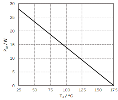
Figure 4. Dissipated power curve
