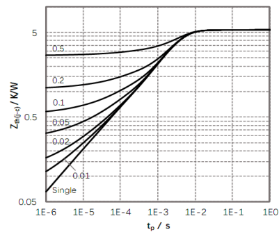
Figure 8. Transient thermal impedance
