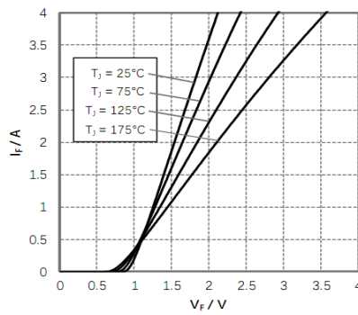
Figure 1. Forward Characteristics
