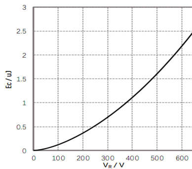
Figure 7. Capacitance stored energy
