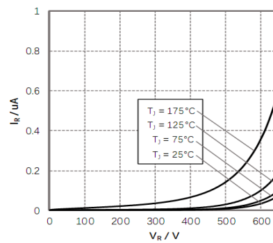
Figure 2. Reverse Characteristics
