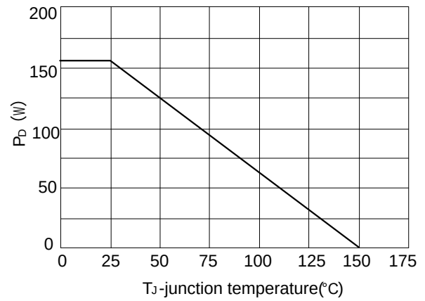
Figure 8 : Power de-rating
