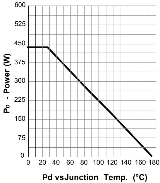
Power Capability
