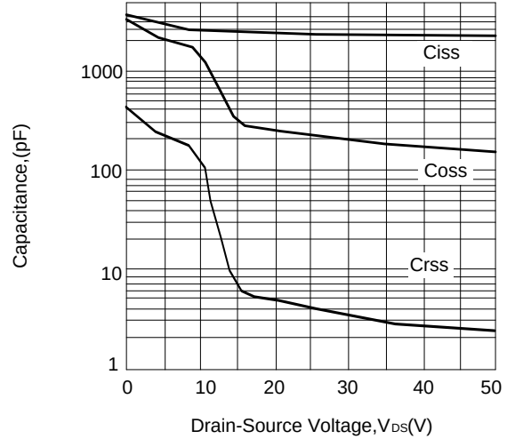
Figure 4: Capacitance Characteristics
