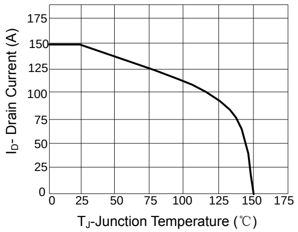
Figure 10: Current de-tating
