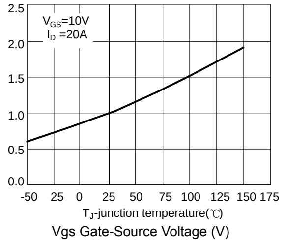
Figure 4: Rdson-junction temperature
