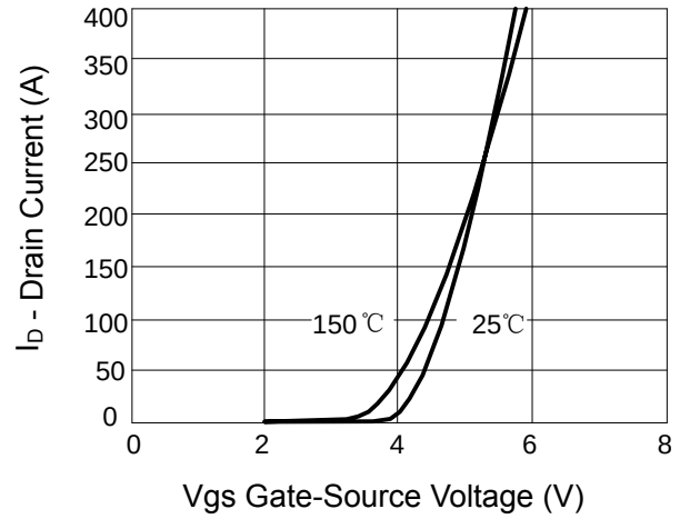
Figure 2: Transfert characteristics
