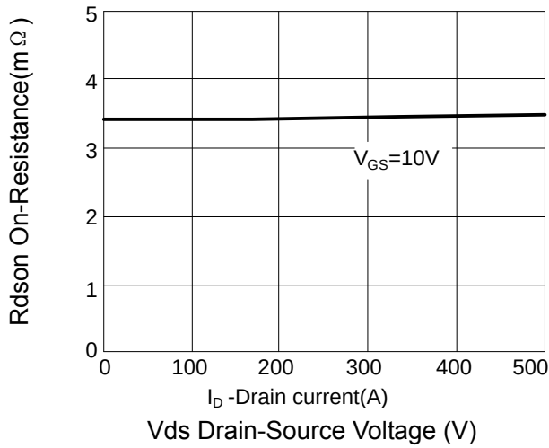
Figure 3: Rdson-drain current
