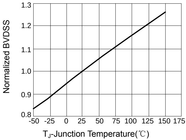
Figure 9: BVDss vs jinction temperature
