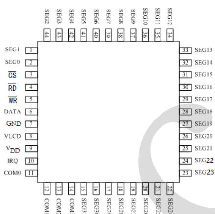
QFP44
