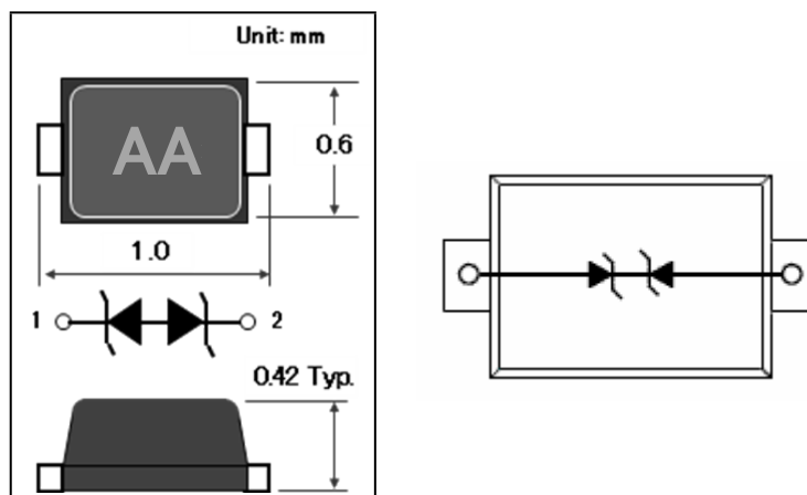
Fig -1 Package SOD923
