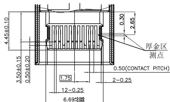
SECTION B-B Scale 1:1
