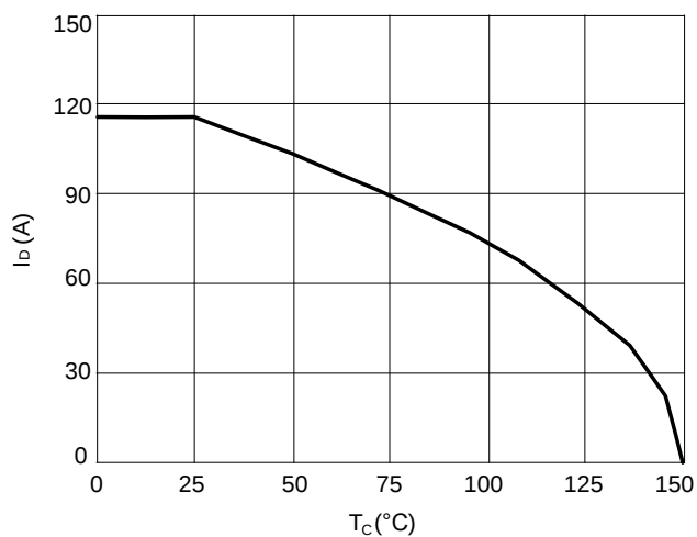
Figure 11: Current De-rating
