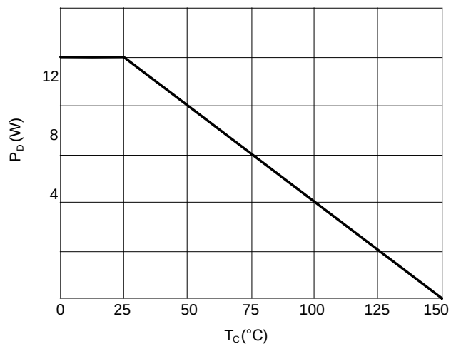
Figure 10: Power De-rating
