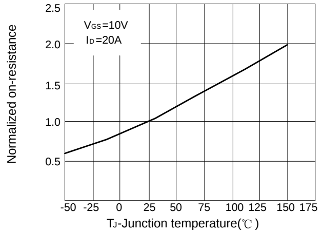
Figure 2: Rdson-junction temperature
