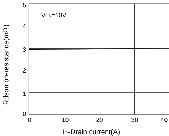
Figure 5: Rdson-drain current
