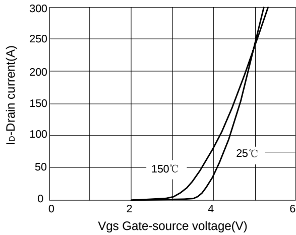
Figure 3: Transfer characteristics
