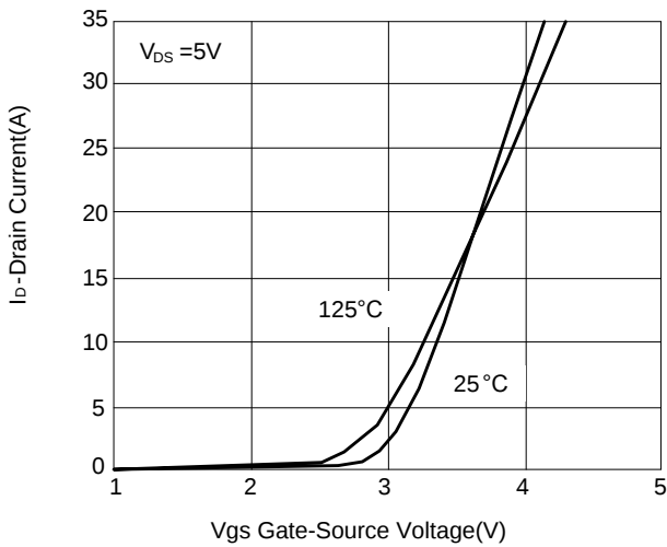
Figure 3: Transfer Characteristics
