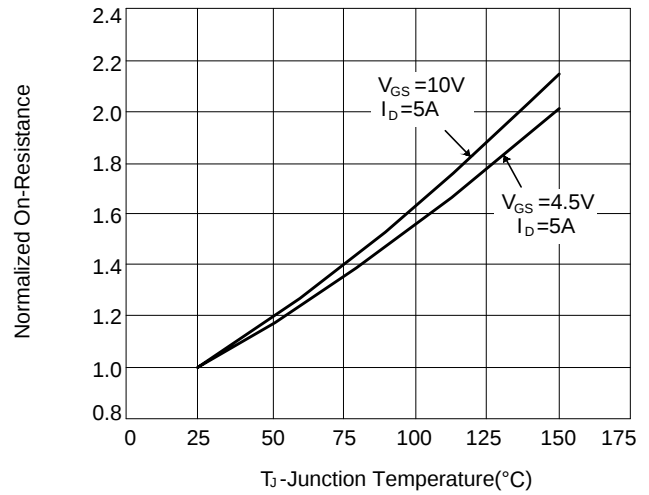
Figure 2: Rdson-Junction Temperature
