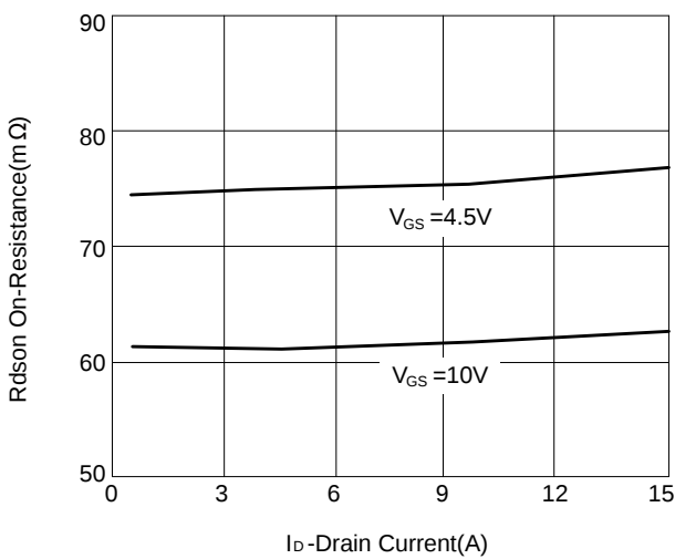
Figure 5: Rdson-Drain Current
