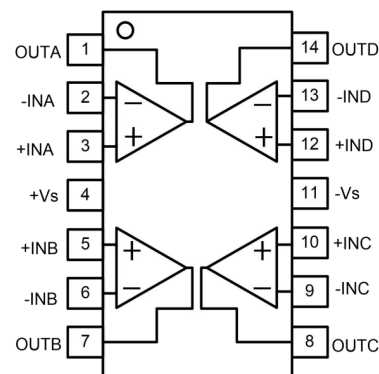
LMV324
